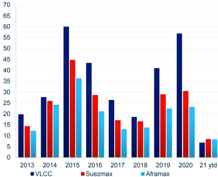
Avg TC results in US$ k/d for crude carriers 2012- 2021
